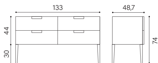
Madia 4 Cassetti / 4 drawer Sideboard
