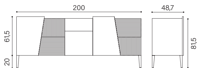
Madia 5 ante battenti e cassetto / Sideboard 5 hinged doors and 1 drawer
